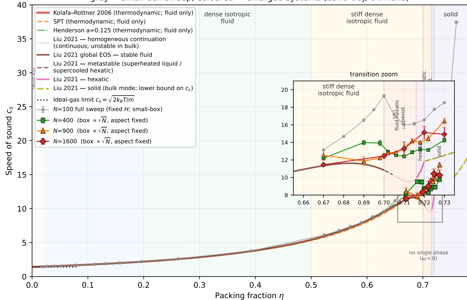
Hard-disk c_s(\eta) with fixed-aspect-ratio finite-size correction grey = small-box sweep; coloured = enlarged systems (2540 traj, 0 invalid)
